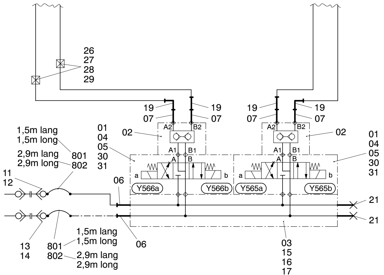
Verbolzung links Pin locking lh
