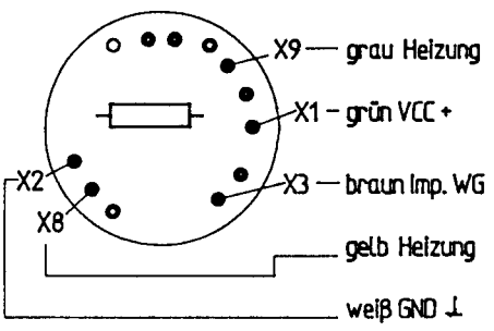
Verdrahtung Pos. 7 Junction, fig. no. 07
